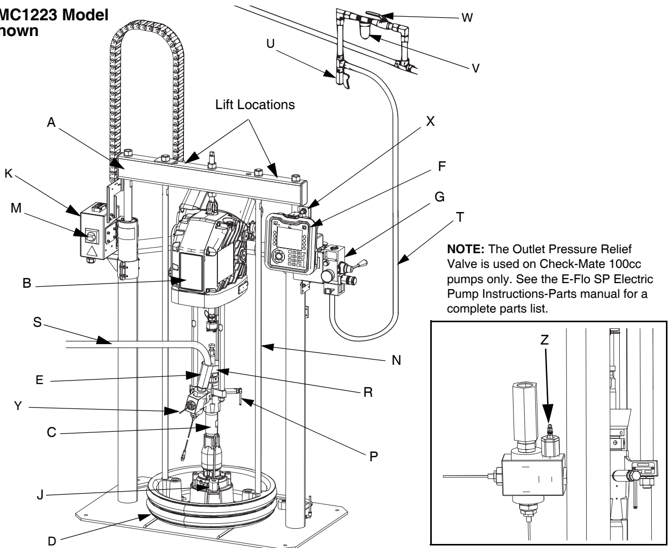
FIG. 1: Typical Installation
