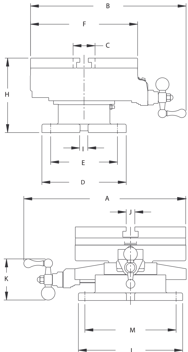
Figure 1 - Dimensions
