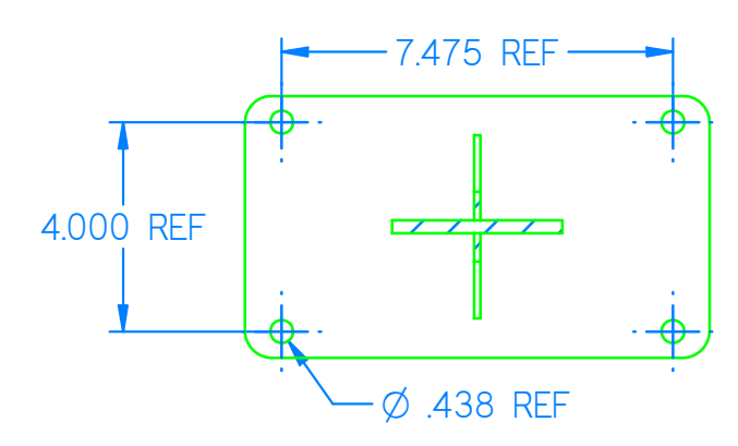
SECTION A-A MOUNTING VIEW (1:4 SCALE)
